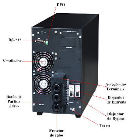
Fig 1- 2: Painel Traseiro
