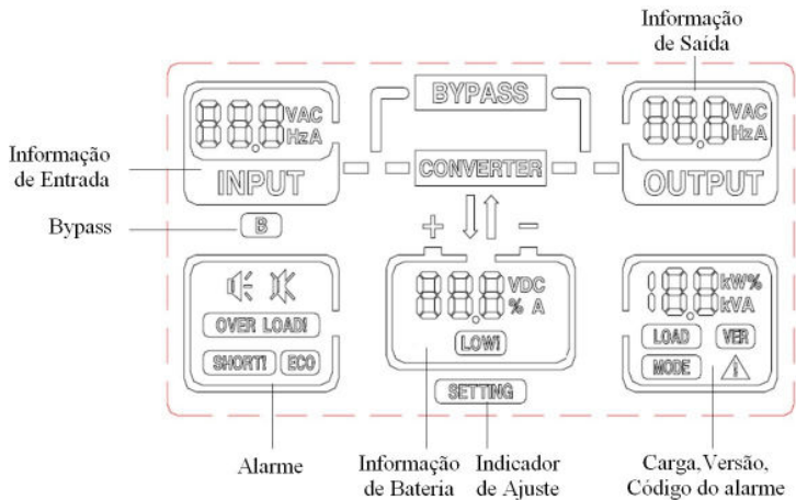
Fig 3- 2: Menu LCD
